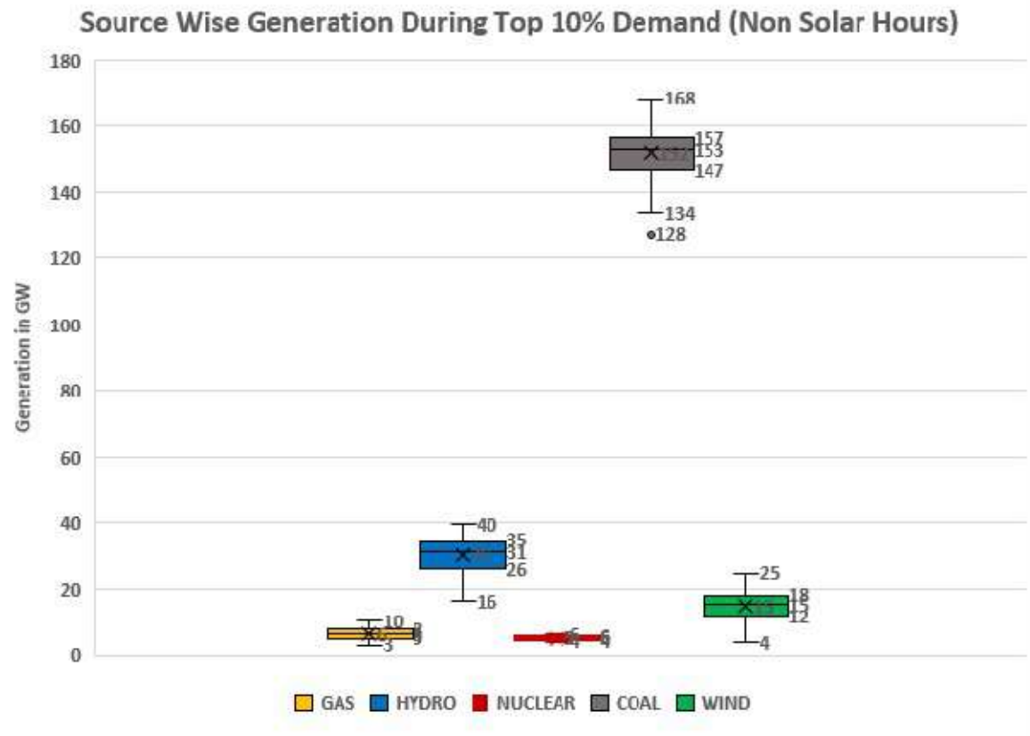
Figure 19(c): Source Wise Generation During Top 10% Demand (Non-Solar Hours) in FY 2023-24
