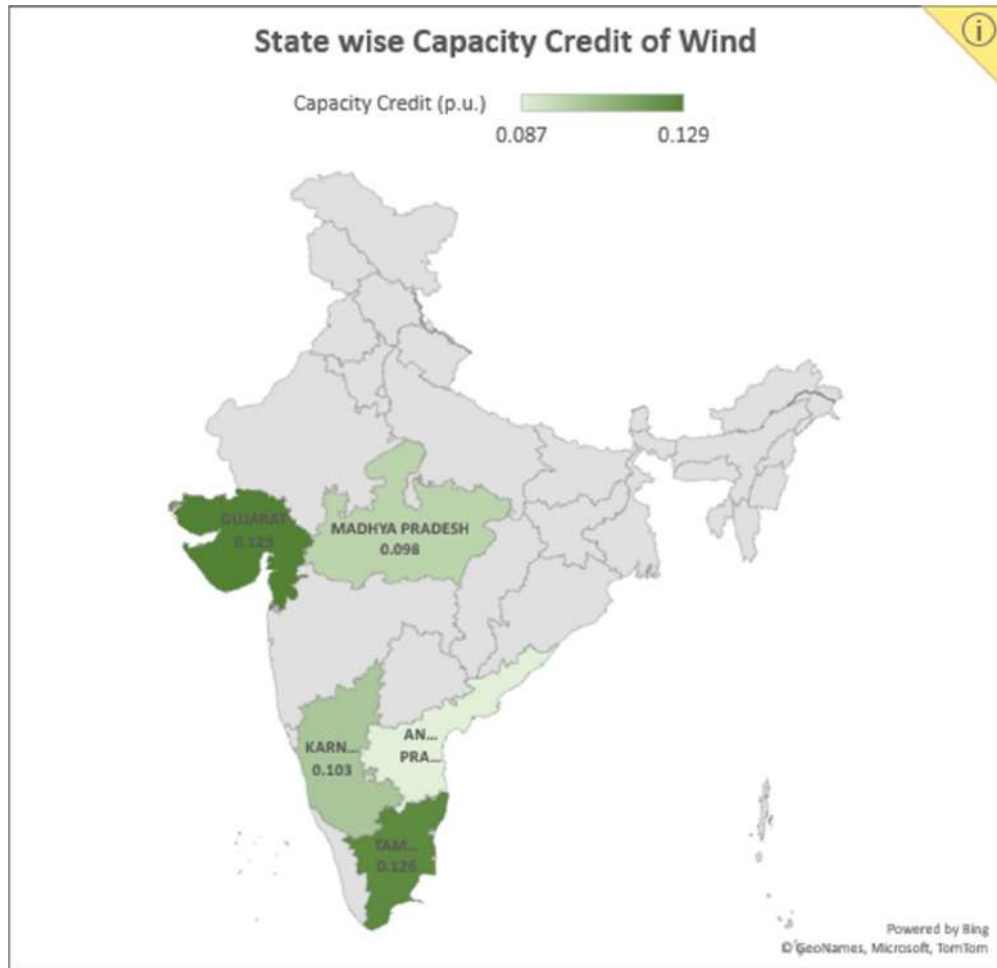
Figure 15: State Wise Capacity Credit of Wind
