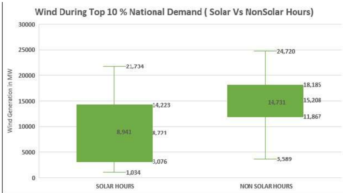
Figure 17: Availability of Wind during Top 10% National Demand (Solar vs. Non-Solar Hours)
