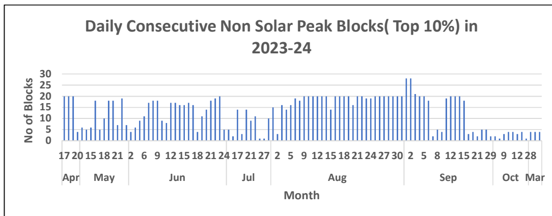
Figure 22: Daily Consecutive Non-Solar Peak Blocks (Top 10%) in 2023-24
