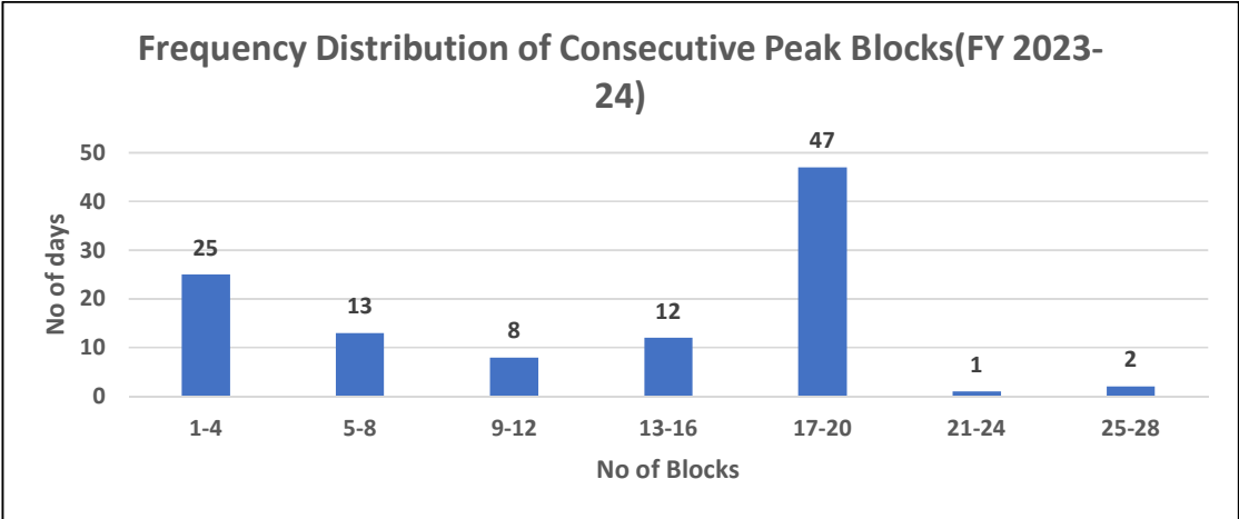
Figure 23: Frequency Distribution of Consecutive Non solar Peak Blocks (Top 10%) (FY 2023-24)
