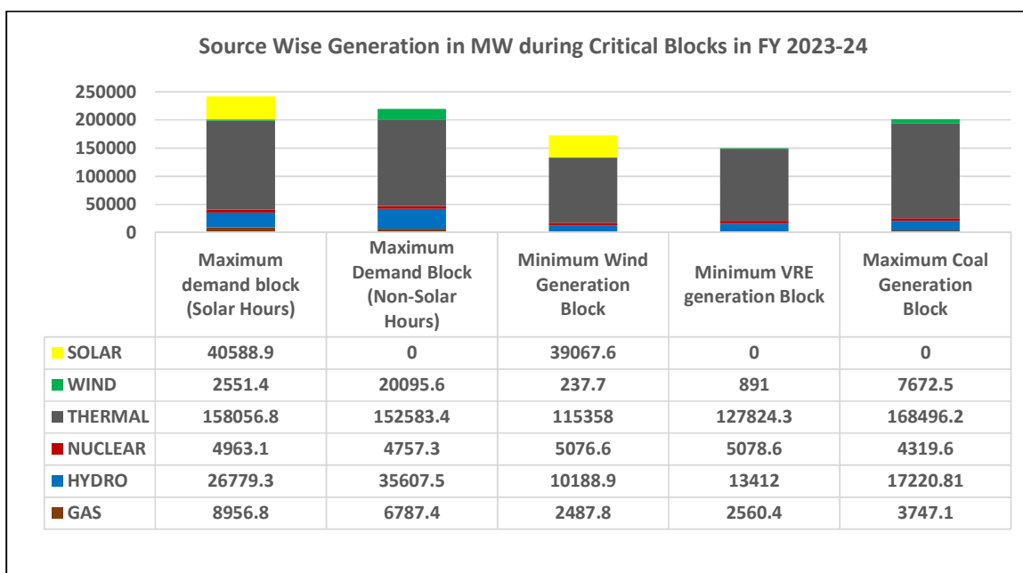
Figure 5: Source-wise Generation During Critical Blocks in FY 2023-24
