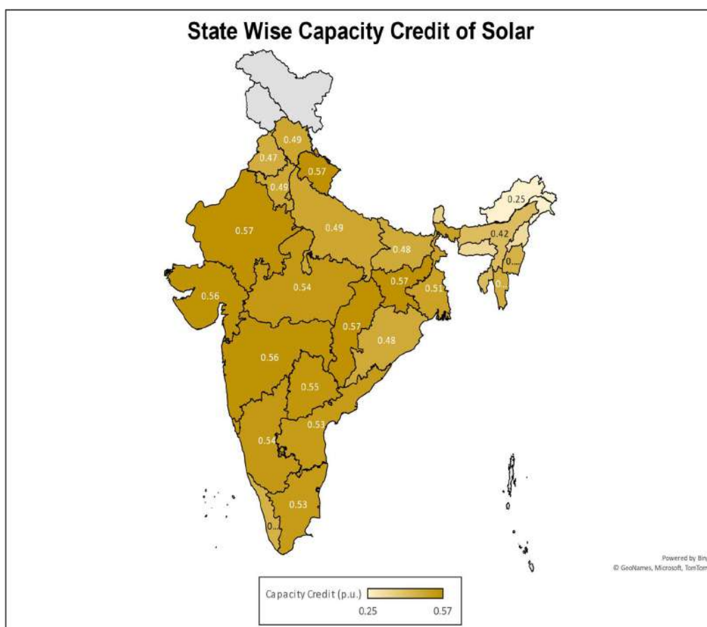
Figure 14: State Wise Capacity Credit of Solar
