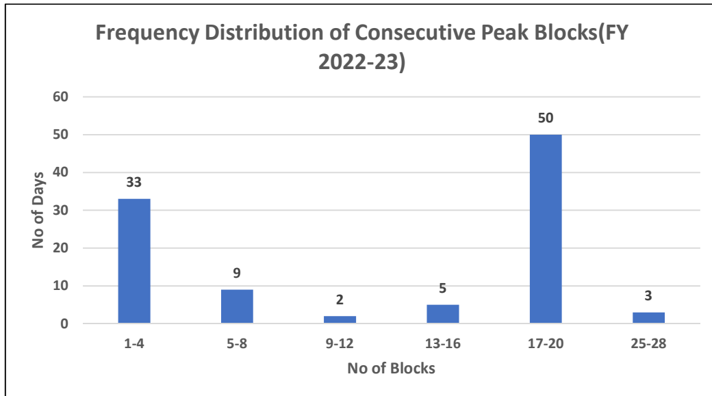
Figure 25: Frequency Distribution of Consecutive Non solar Peak Blocks (Top 10%)(FY 2022-23)
