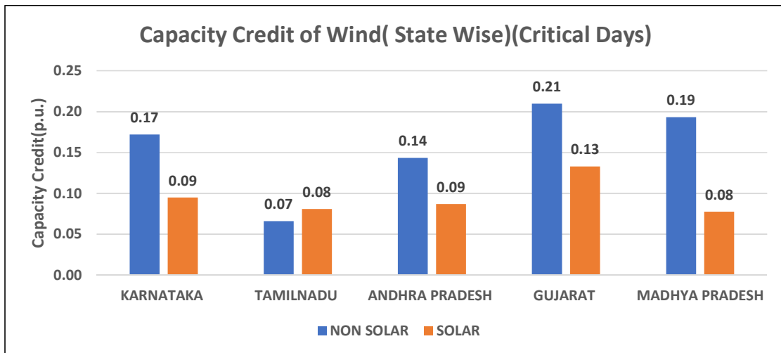
Figure 21: Capacity Credit of Wind (State Wise) (Critical Days)
